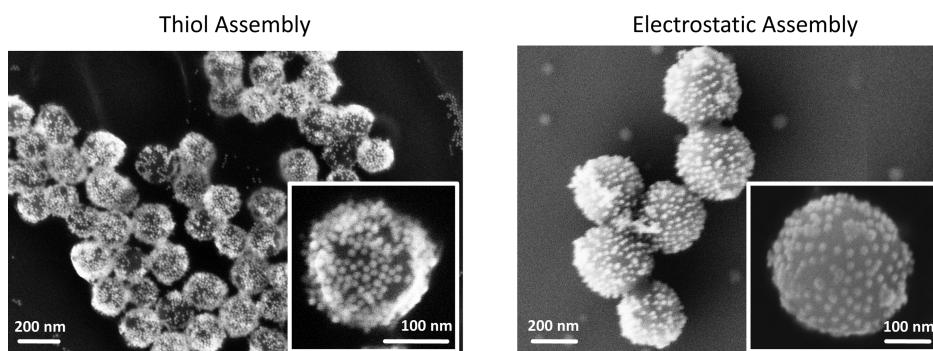
Figure 1. Scanning electron micrographs of fabricated core–shell clusters (for geometrical details, see text). An amorphous arrangement of core–shell clusters of thiol assembly and of electrostatic assembly is shown in the left and right panels, respectively. The inset of both micrographs depicts a zoomed in view showing a single core–shell cluster.
